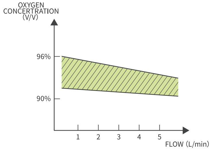
Oxygen concentration under the operational flow
