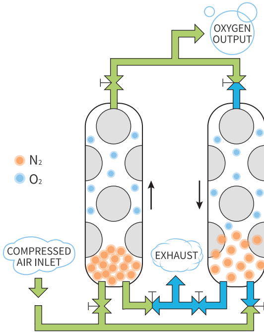
How the molecular sieve works
